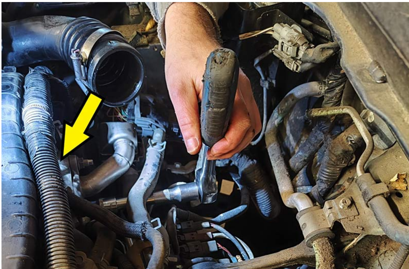
Subaru Forster EGR valve installation position
