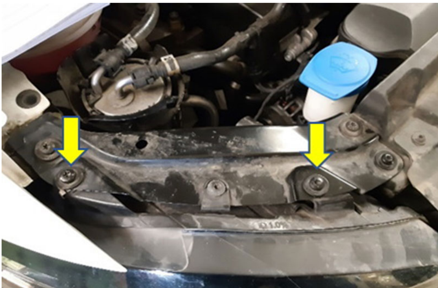
Fastening screws
