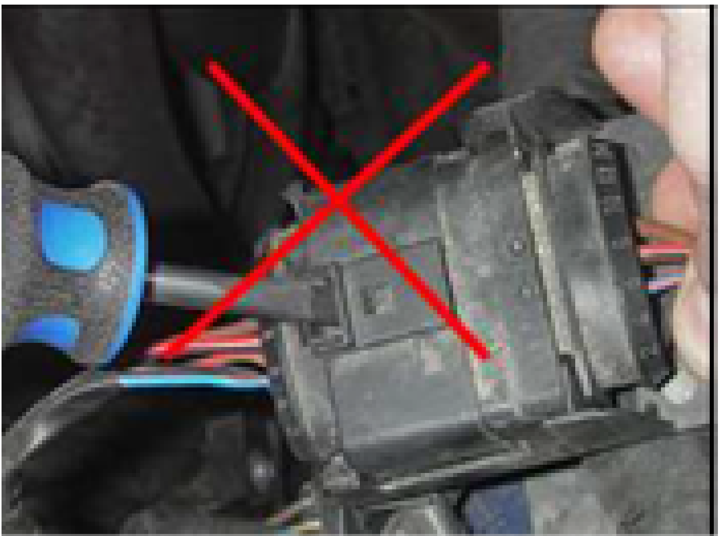
Figure 1.: 14-pin connector
