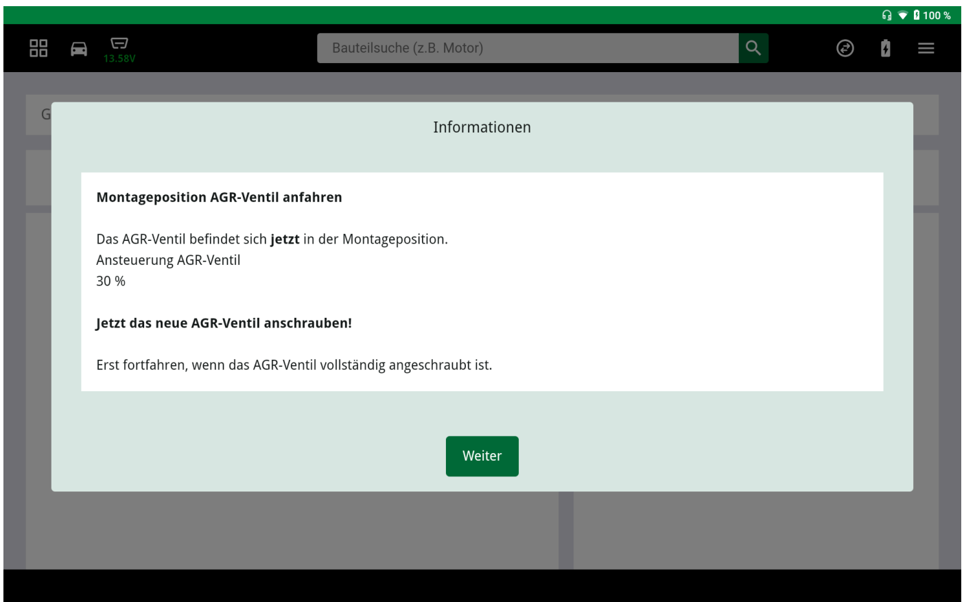
Fig. 5) EGR valve can now be installed
