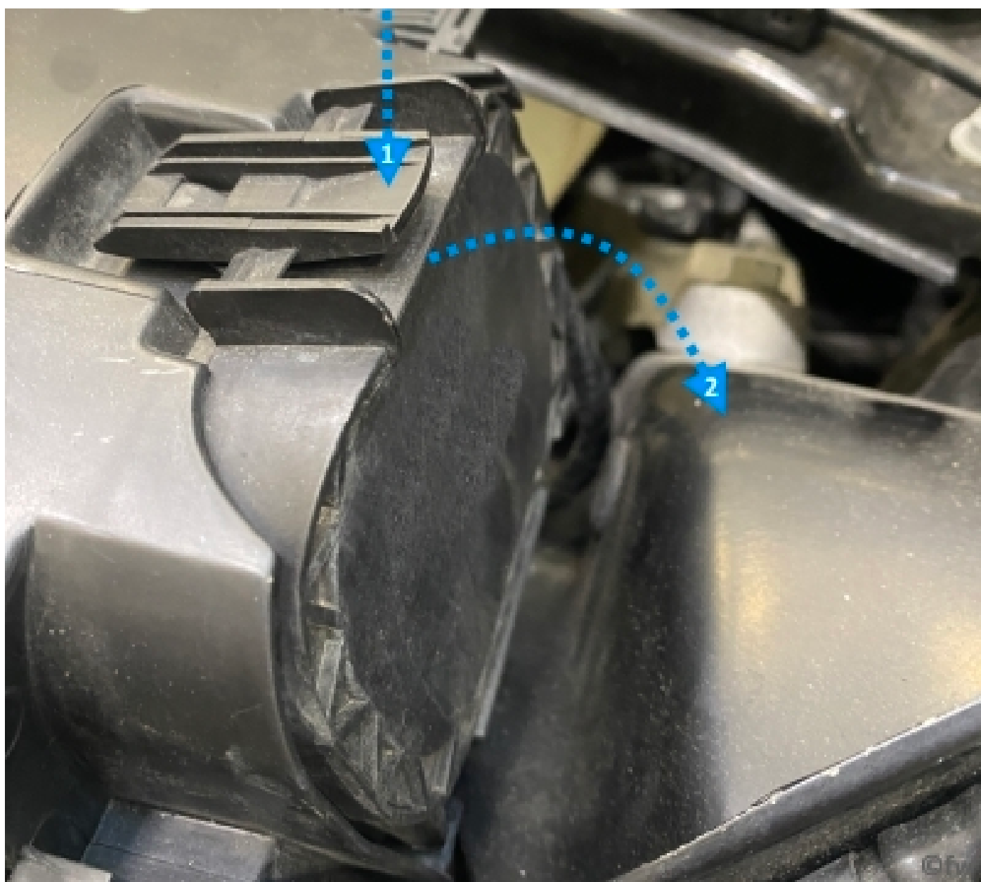
Front view of the Mini R57 lamp cover cap
