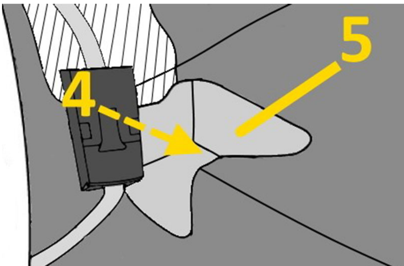
Picture 1: Permanent contact between the plug connection of the side airbag and the seat backrest upholstery
