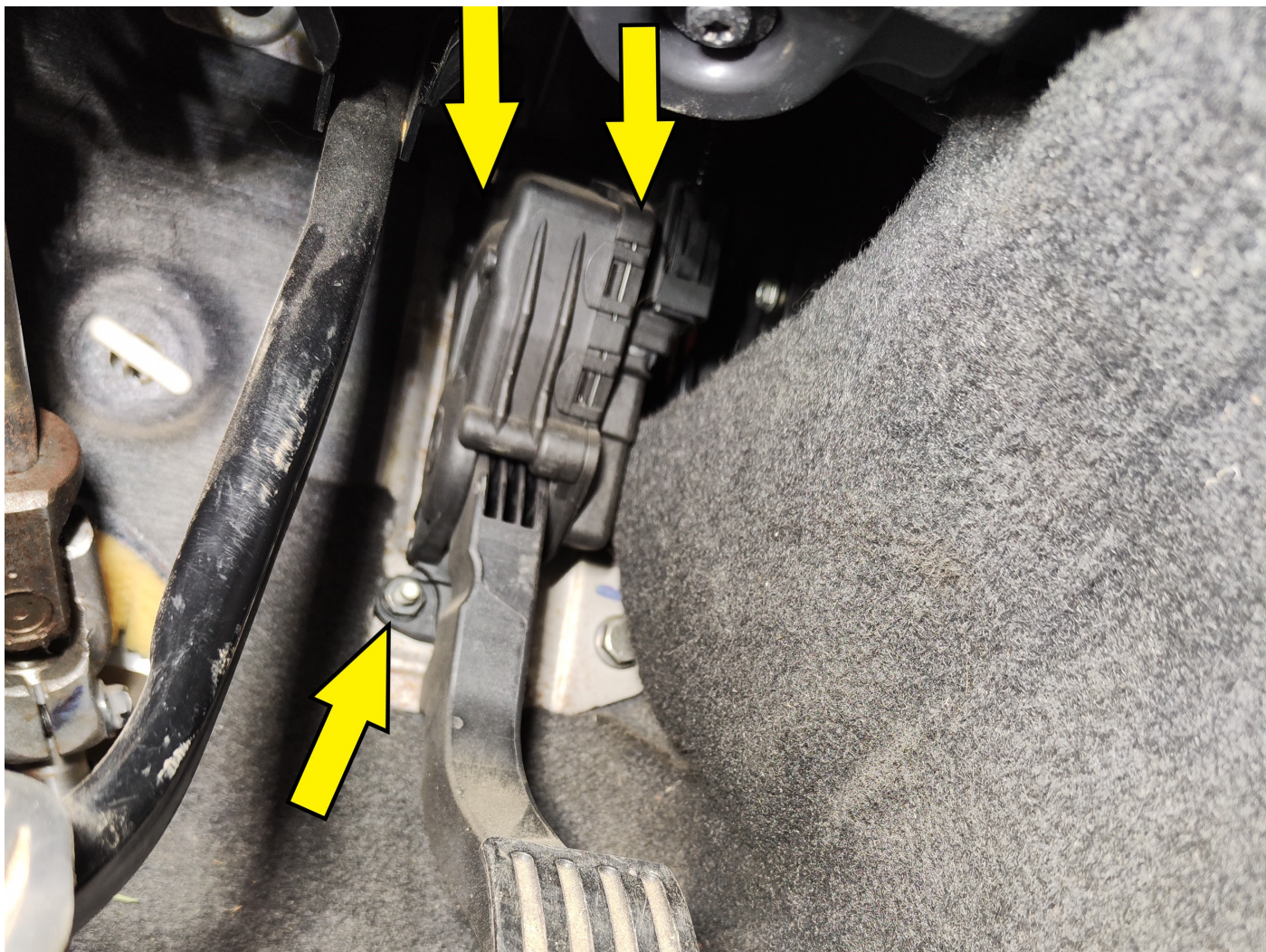
Volvo V50 accelerator pedal
