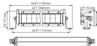
Black Magic 40" Slim Curved Lightbar
