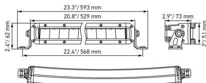
Black Magic 21.5" Double Row Curved Lightbar
