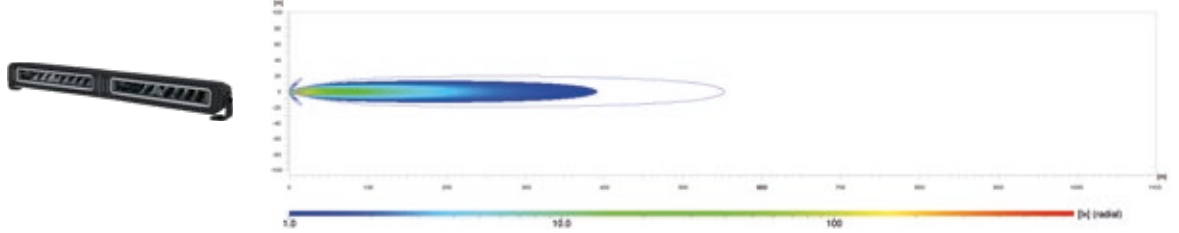
22" Single Twin Lightbar Black Magic Tough Pro | 1FJ 358 550-401 Referentiegetal 40 | ECE- + high-boost-modus | grootlicht
