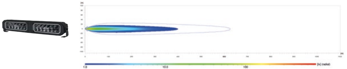
18" Double Twin Lightbar Black Magic Tough Pro | 1FJ 358 550-421 Referentiegetal 40 | ECE- + high-boost-modus | grootlicht
