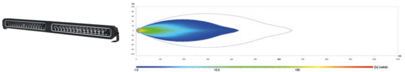
38" Double Twin Lightbar Black Magic Tough Pro | 1FJ 358 550-431 Referentiegetal 50 | ECE- + high-boost-modus | grootlicht
