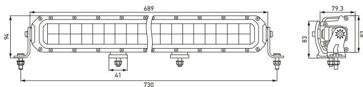
27" Double Row Lightbar Black Magic Tough Pro
