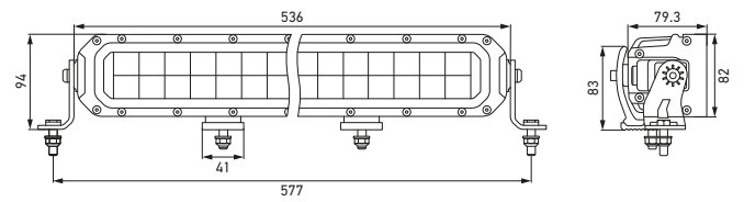
21" Double Row Lightbar Black Magic Tough Pro
