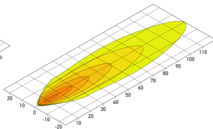
Long-range illumination
