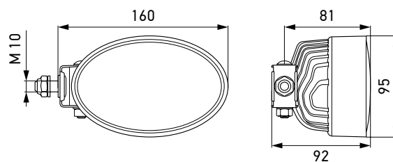
Lateral mounting
