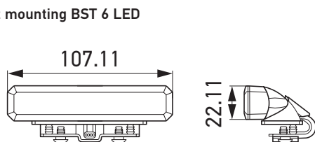
Bracket mounting BST 6 LED
