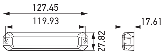
Surface mounting BST 6 LED
