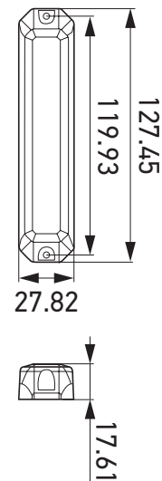
Surface mounting BST-V 6 LED
