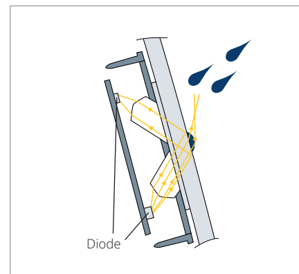
Regensensor
