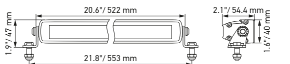
Black Magic Lightbar 20" (Slim)
