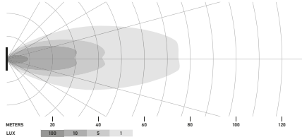
LED Cube SET 2,7", Floodlight
