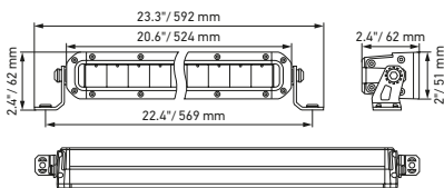
Black Magic 20" Slim Lightbar
