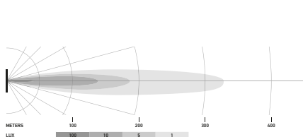
LED Cube SET 3,2", luz puntual
