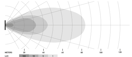
LED Cube SET 3,2", luz difusa
