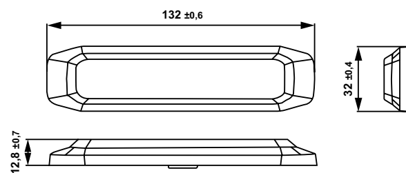
Surface mounting BST-Slim 6 LED
