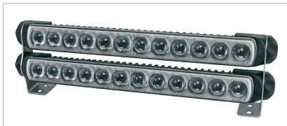
P/N 8HG 958 128-811 HD Double mount stainless steel feet (one pair) to suit RokLUME S700 LED range
