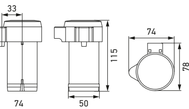
Reservedel | CM40 Kompressor
