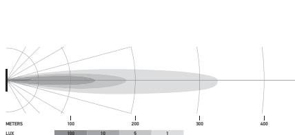
SET LED Cube SET 3.2", faretto
