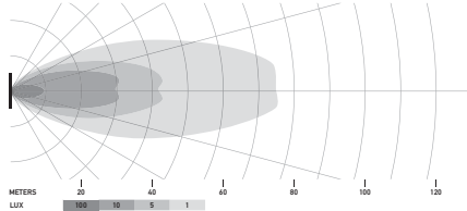
LED Cube SET 2,7", Flutlicht
