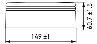
Fixed mounting (F)
