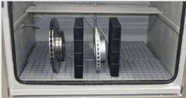
Test setup before and during testing
