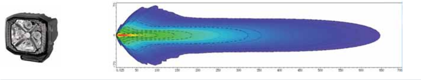
HELLA X-Treme 4.3 inch - Spot
