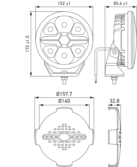
Round cover, 6 inch (8XS 358 198-031, optional accessories)
