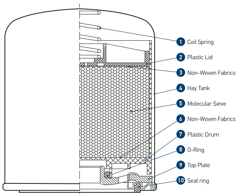
Product sketch
