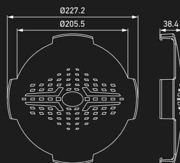
Ronde afdekking, 9 inch (8XS 358 198-011, optionele accessoire)
