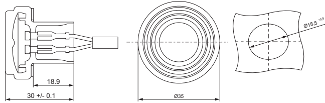
Plastic Housing
