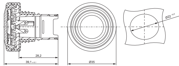
Rubber Housing
