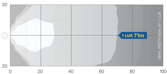
Ultra Beam X-Powerpack XGD 2.5m high at 10°
