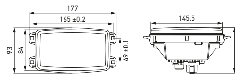
Flush mounting
