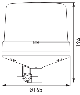
Pipe socket mounting (P)
