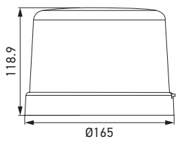
Fixed mounting (F)
