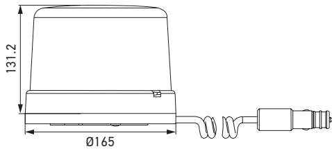
Magnet mounting (M)
